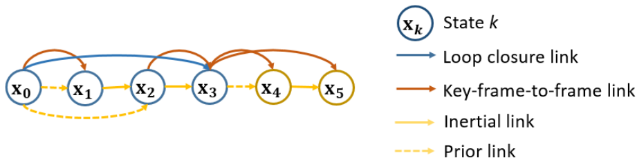
Fig. 3: Graph representation of variables ( \mathbf{x}_k = [\mathbf{p}_{b_k}^w, \mathbf{v}_{b_k}^w, \mathbf{q}_{b_k}^w, \mathbf{b}_a^{b_k}, \mathbf{b}_\omega^{b_k}] ) and constraints (inertial links, prior links, keyframe-to-frame links and loop closure links). See Sect. 6 for details about variables and constraints.
