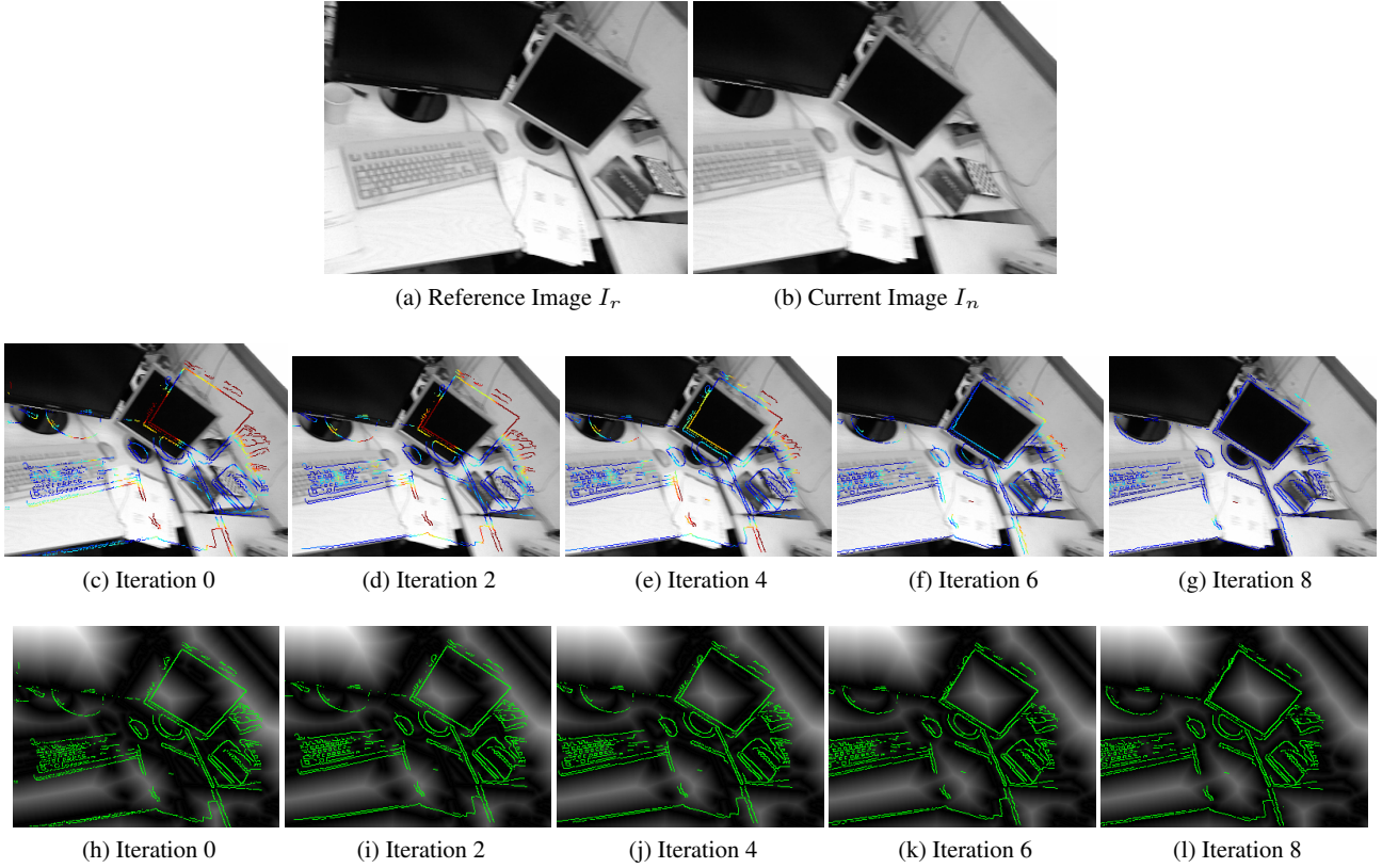
Fig. 4: Reprojections of edge-pixels in the reference frame onto the current frame as the Gaussian-Newton optimization progresses. The middle row shows the reprojections on the current gray image. They are false colored to represent v_{e_i}(\xi) . The last row shows reprojections on the distance transform image of the edge-map of the current frame. Note that the current frame and the reference frame are about 160 ms apart (5 frames) and the Gaussian-Newton method progress is shown without pyramids, with the initial guess as the identity. Viewing in color is recommended.
