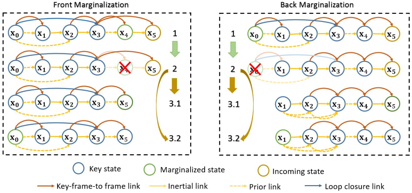
Fig. 5: The process of our two-way marginalization, which marginalizes all the available information (motion estimates from edge alignment, inertial measurement, loop closure relation and prior) into a new prior and maintains bounded computational complexity. Front marginalization marginalizes the second newest state, while back marginalization marginalizes the oldest state within the sliding window.
