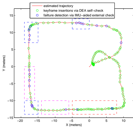
Fig. 7: The estimated trajectory of a walk around a circular path with different lighting conditions.
