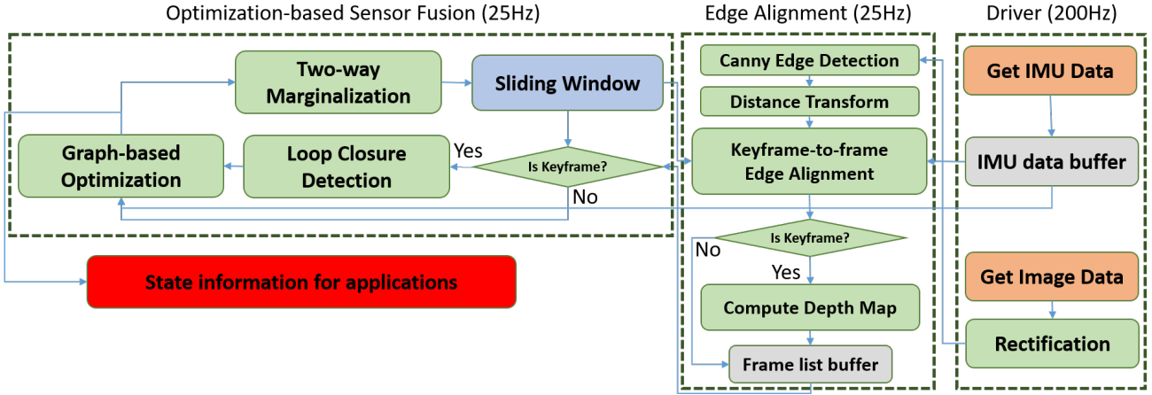
Fig. 2: The pipeline of our proposed system. It consists of three modules running in separate threads to ensure real-time availability of state estimates (denoted as three dashed boxes). The driver thread runs at 200 Hz, the edge alignment thread runs at 25 Hz, and the optimization-based sensor fusion thread runs at 25 Hz.
